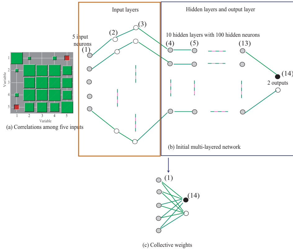
Figure 5: Correlation coefficients among five input variables (a), two-step information augmentation (b), and collective weights (c) for the snack food selection data set. The size of the squares represents the magnitude of correlations; green and red ones show positive and negative correlations, respectively.
