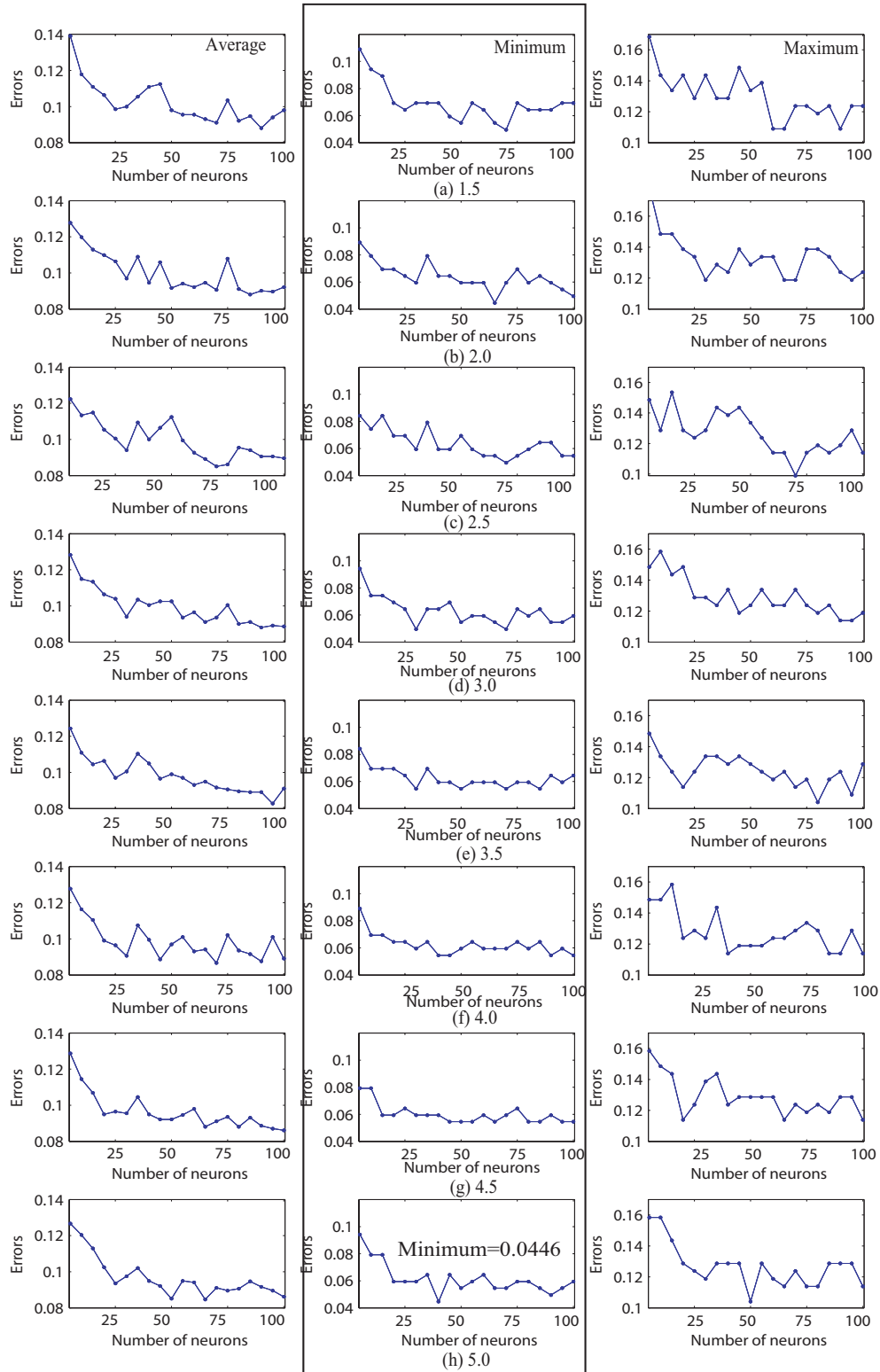
Figure 6: Generalization errors in terms of average (left), minimum (middle), and maximum (right) when the constant \theta for the third layer increased from 1.5 (top) to 5 (bottom) for the snack food data set.
