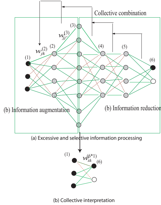
Figure 4: Reduction from the conventional weights (a) to the collective weights (b).
