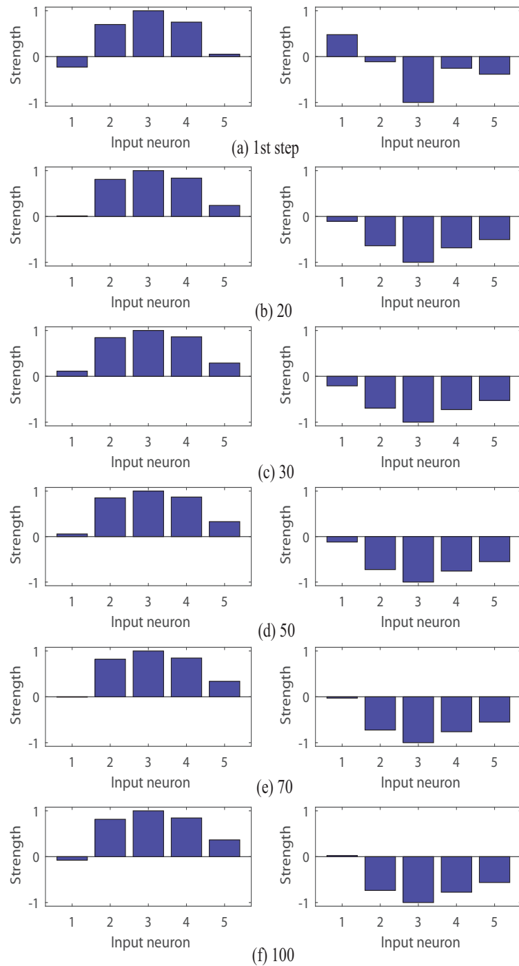
Figure 8: Collective weights with 90 neurons in the second layer and with \theta = 3.0 with the worst generalization errors into the first and the second output neuron from the first learning step (top) to the 100th learning step (bottom) for the snack food data set.
