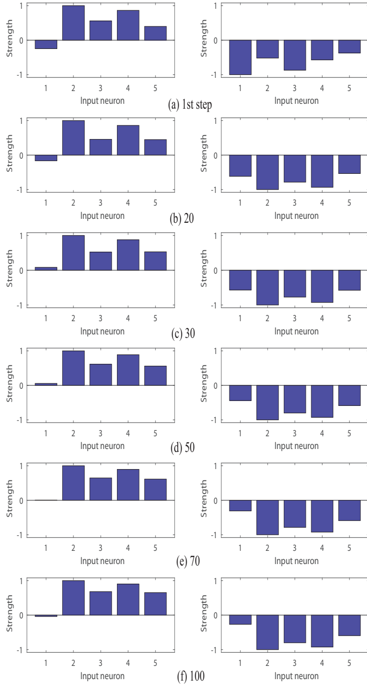
Figure 7: Collective weights with 95 neurons in the second layer with \theta = 3.5 with the best generalization performance into the first and the second output neuron from the first learning step (top) to 100th tenth learning step (bottom) for the snack food data set.
