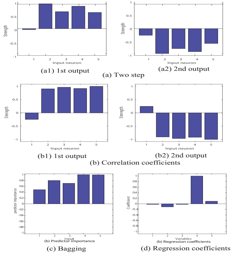
Figure 9: Strength of collective weights into the first and second output by the present method with the best generalization performance (a), correlation coefficients between inputs and targets (b), prediction performance by the bagging method (c), and regression coefficients by the logistic regression analysis (d) for the snack food data set.
